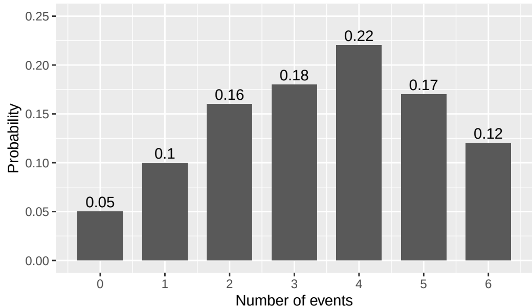
A probability mass function
