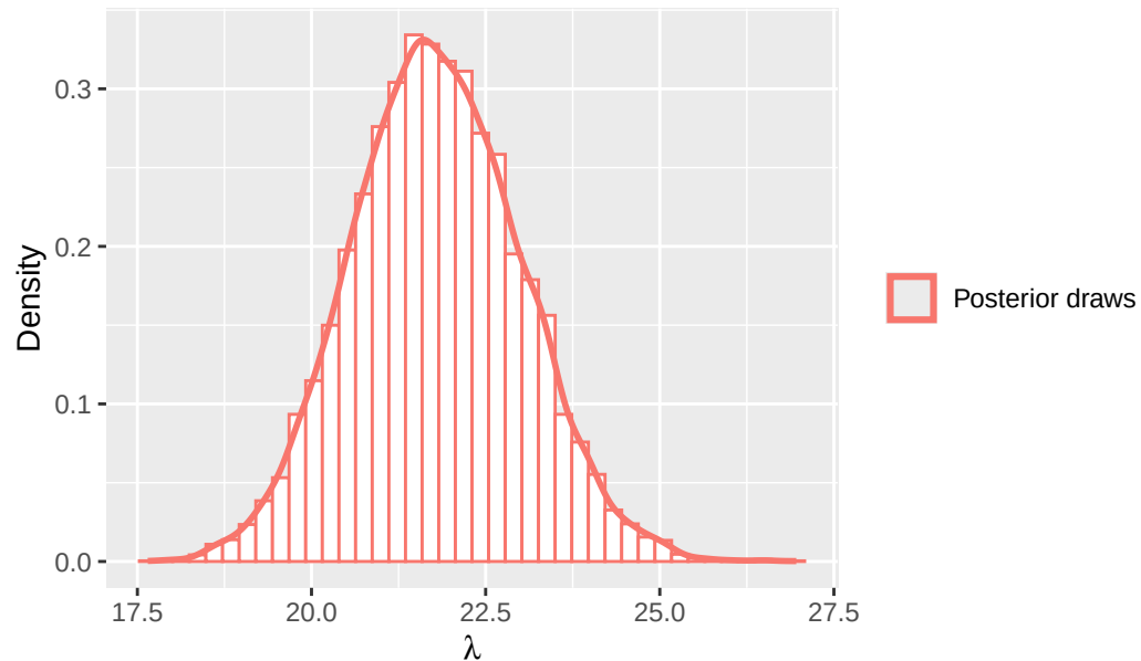
Posterior distribution for the average number of calls per night
