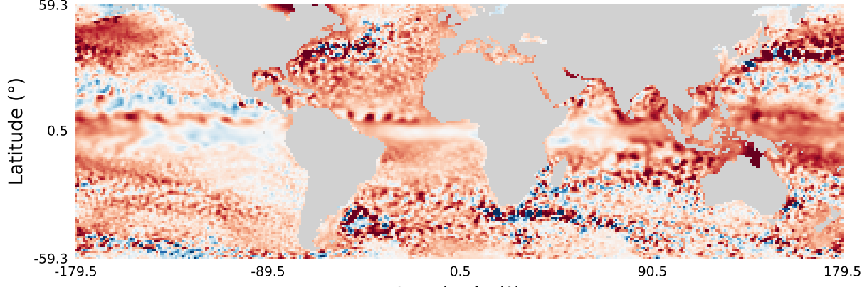
D → observations: inferred-state persistence
