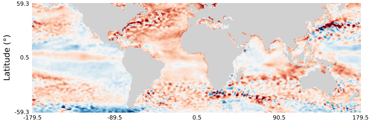
Adapter only
