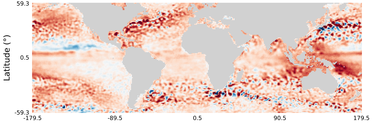
Observation-only scratch
