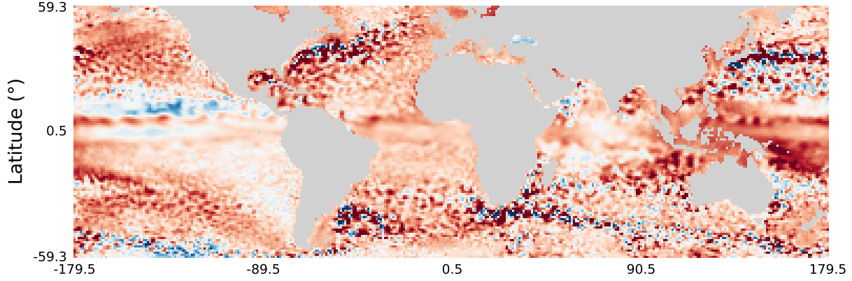
Full fine-tuning
