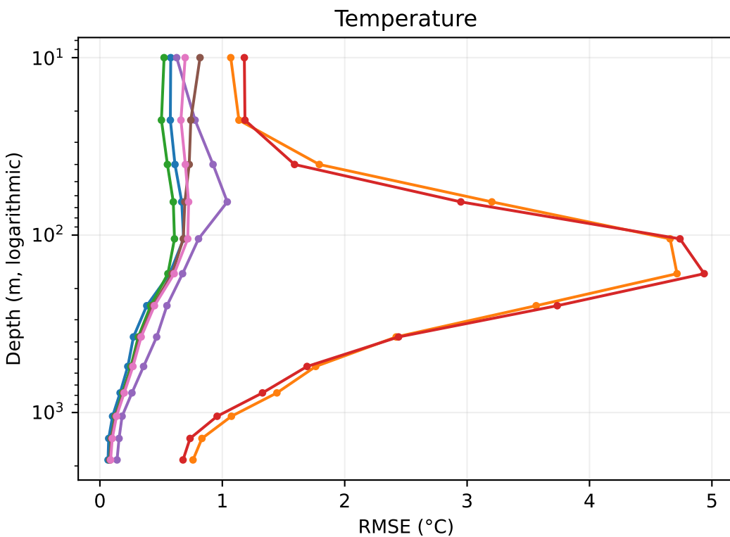
Held-out 2015-2022 monthly forecast T/S against IAP
