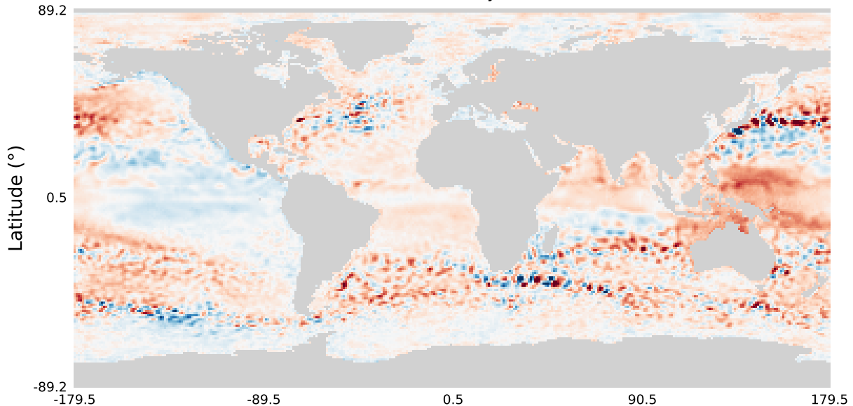
U-multitask-early-fine
