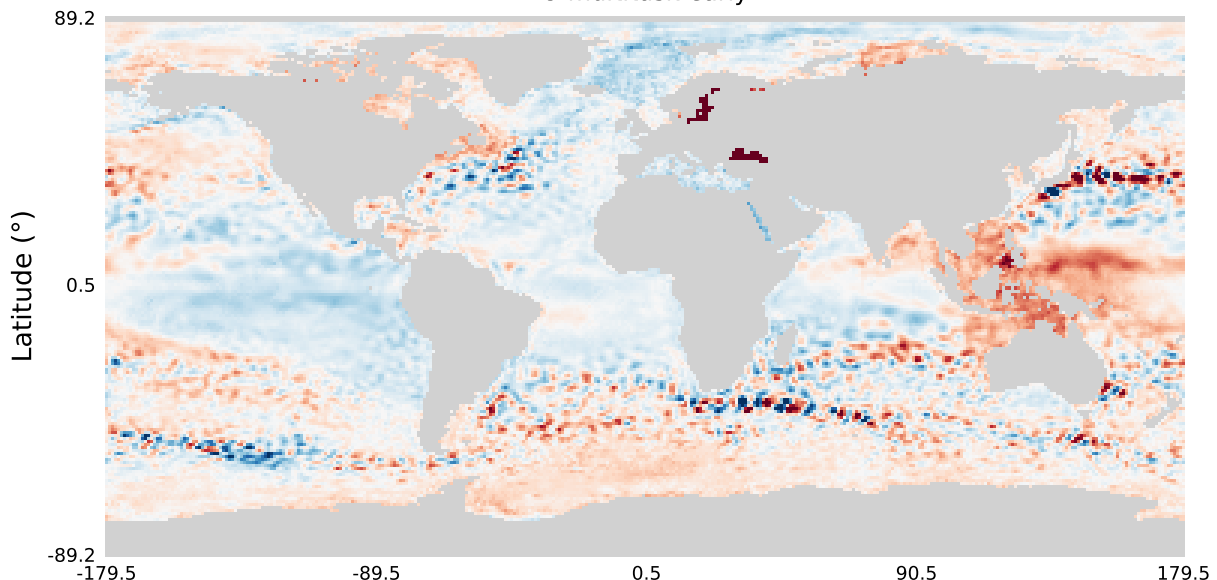
U-multitask-early-latent
