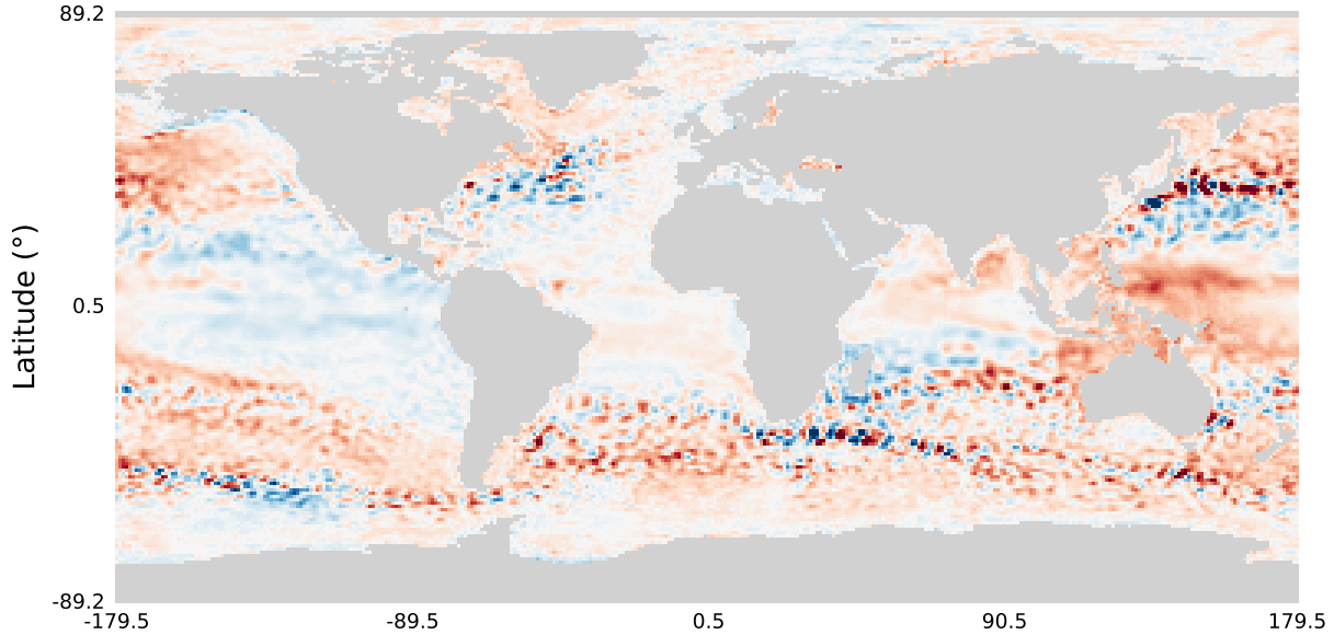
U-multitask-early-fine-latent
