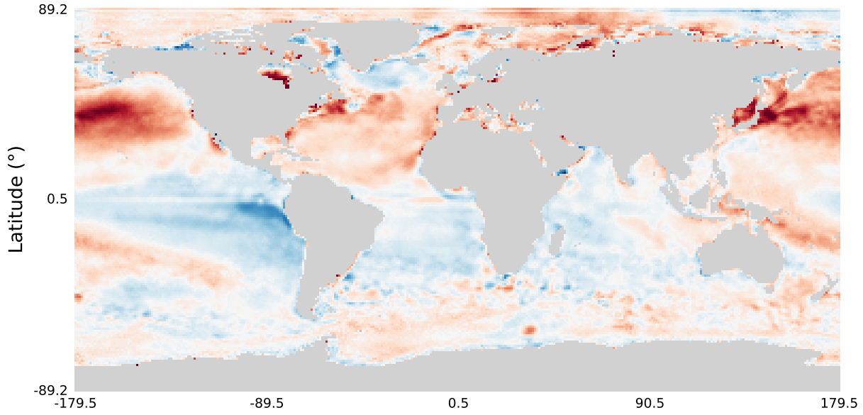
U-patch-truth
