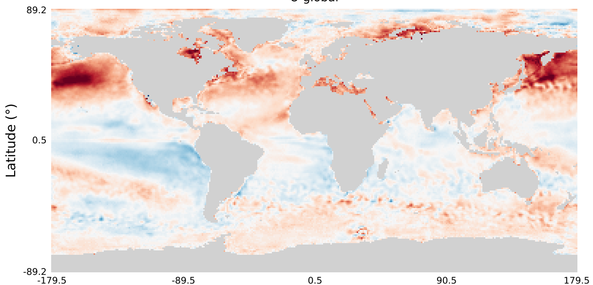
U-multitask
