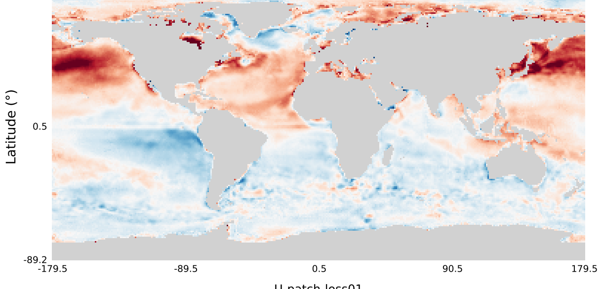
U-patch-loss01
