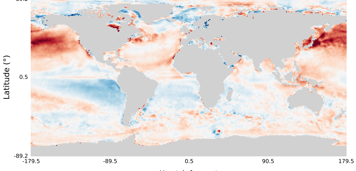
U-patch-forecast
