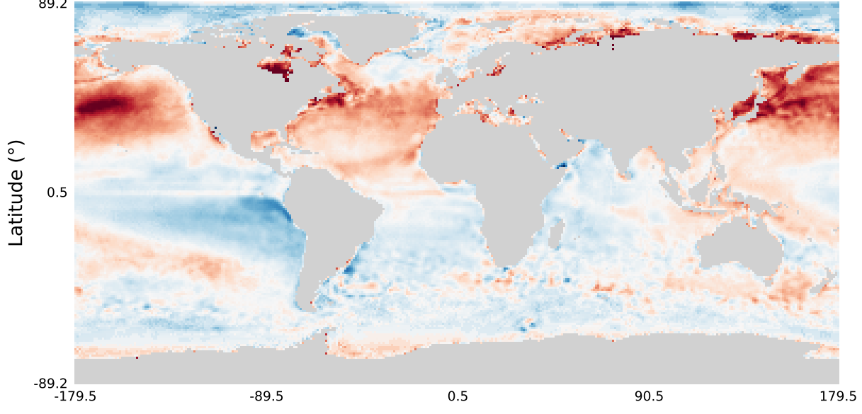
U-patch-detach
