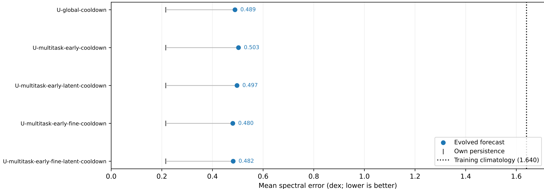
Cooldown models · Original 5 / 15 / 30-day spectral score SST + ADT + EKE · 3 regions · 96 held-out monthly origins
