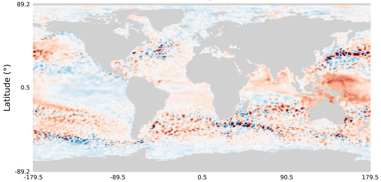
U-multitask-early-fine-latent-cooldown
