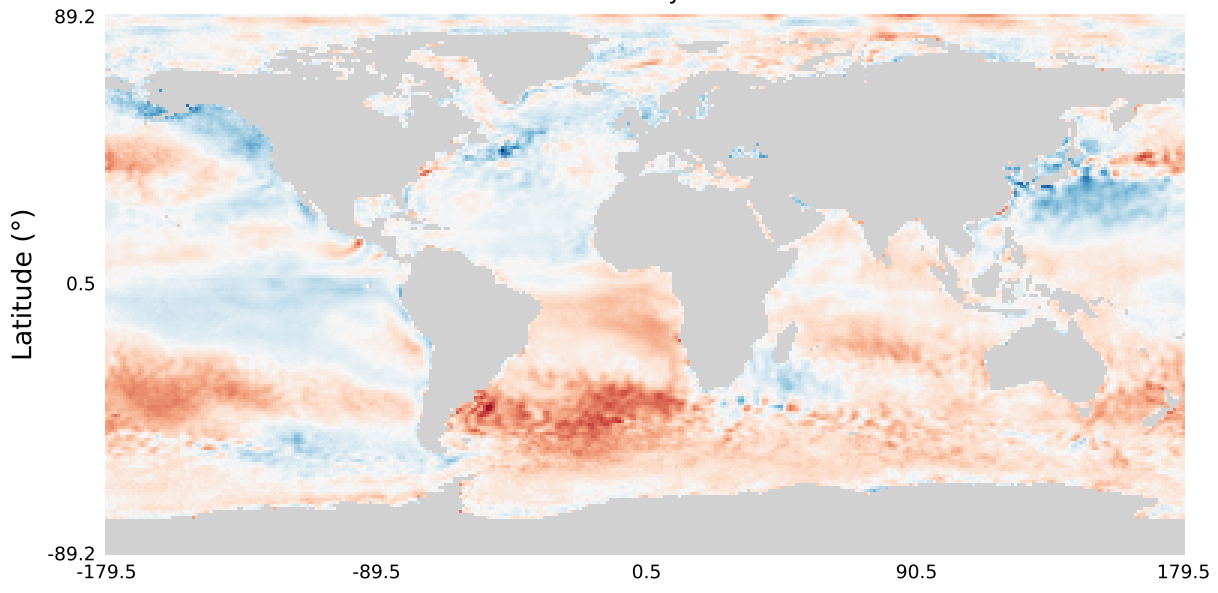
U-multitask-early-fine-latent-cooldown
