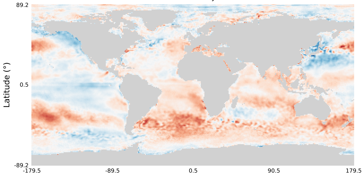
U-multitask-early-fine-cooldown
