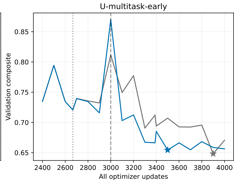
Matched learning-rate cooldown — one seed; lower is better; stars select checkpoints
