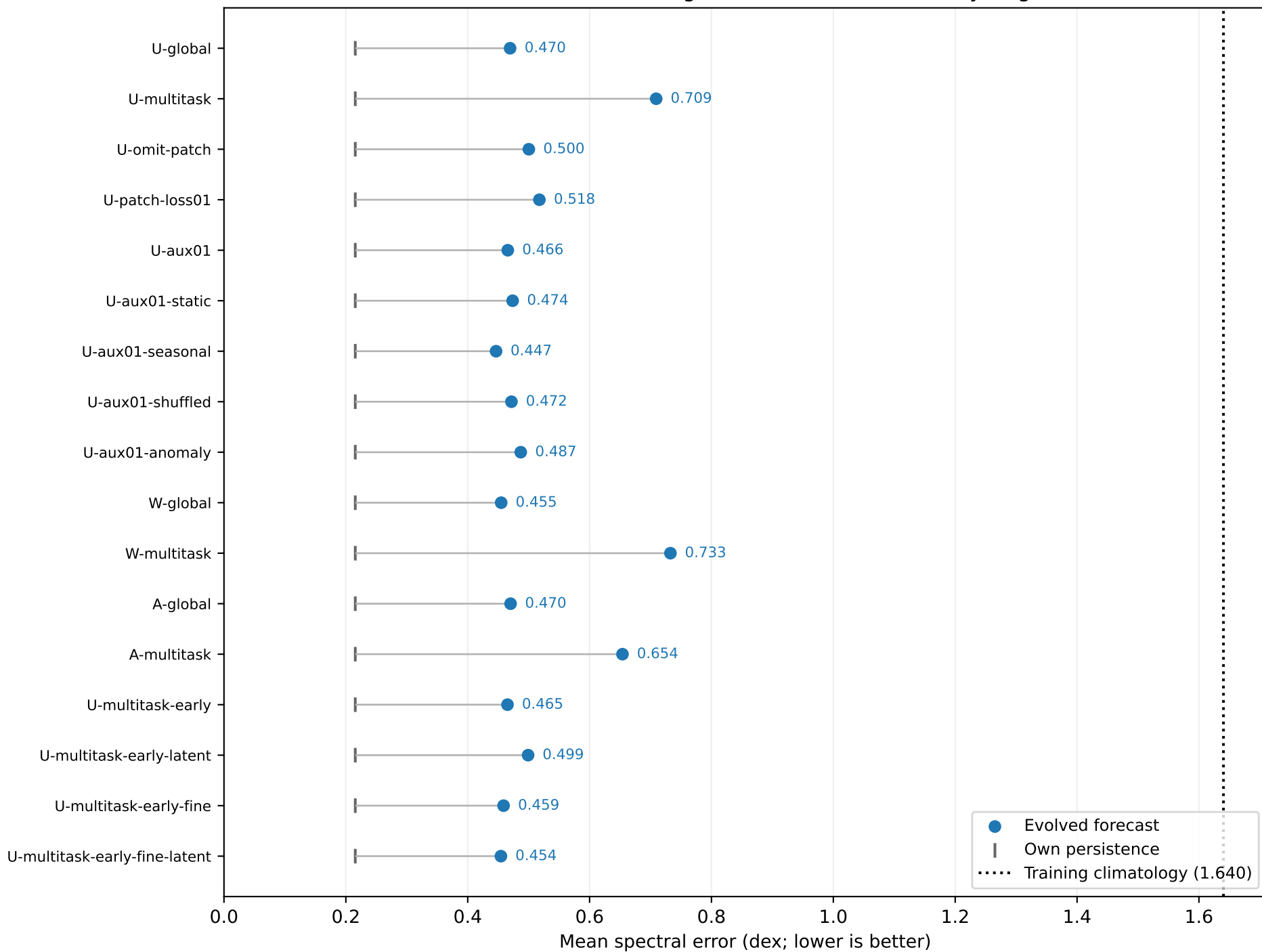
Original 5 / 15 / 30-day spectral score SST + ADT + EKE · 3 regions · 96 held-out monthly origins
