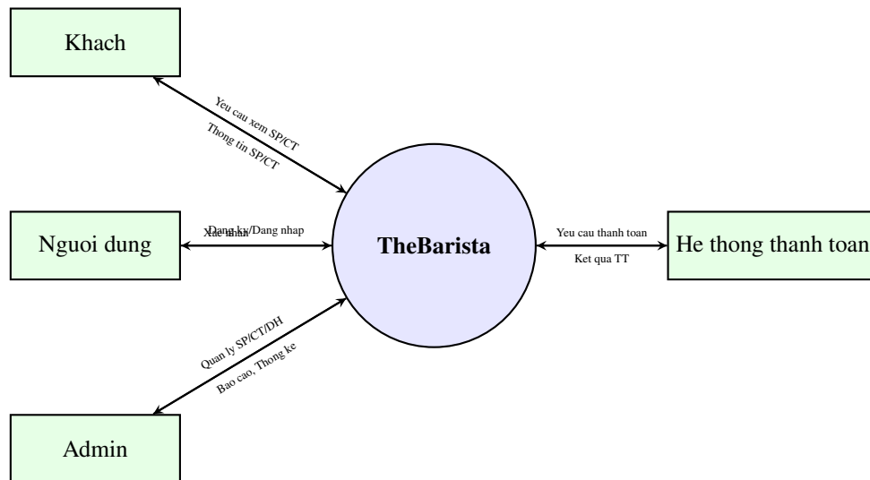
Hình 4.5: Data Flow Diagram Level 0 - Context Diagram
