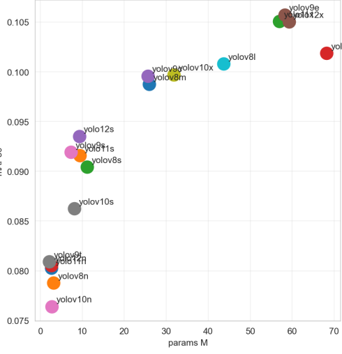
Model Size vs mAP50
