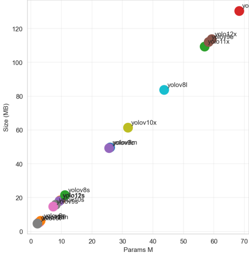
Params vs Model Size MB
