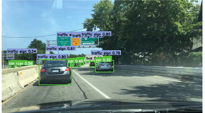
Prediction (21 objects)
