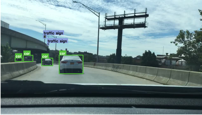
Sample #5: d2c4249f-4568f6ac.jpg
