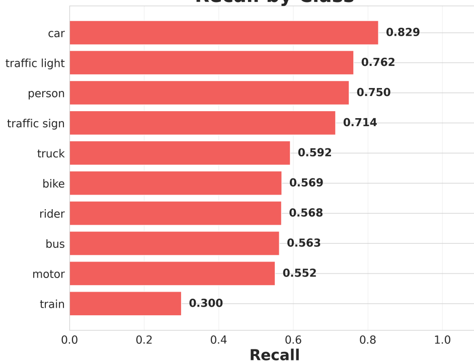
Recall by Class
