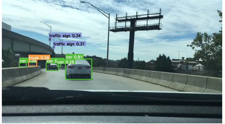
Prediction (7 objects)
