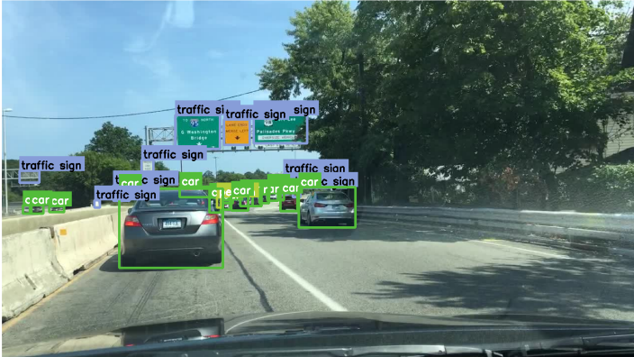
Sample #6: cde381ce-f69c7cf2.jpg
