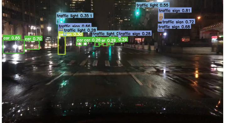
Prediction (20 objects)
