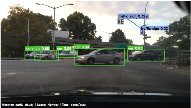
Prediction (8 objects)
