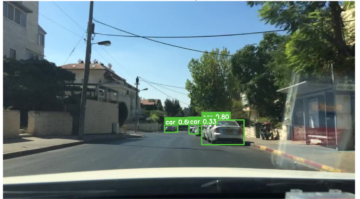
Prediction (3 objects)
