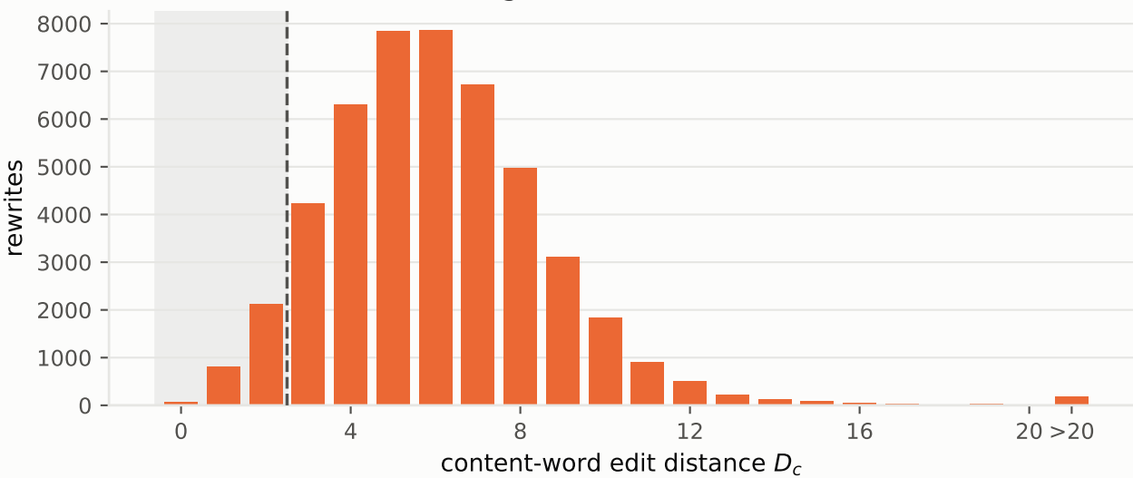
Qwen3-32B (n = 48,000 generated rewrites · D_c \leq 2 : 6.2%)
