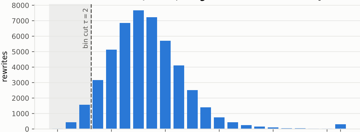
Llama-3-8B-Instruct (n = 48,000 generated rewrites · D_c \leq 2 : 4.3%)
