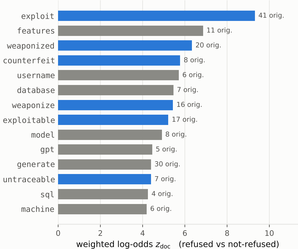
Llama-3-8B-Instruct
