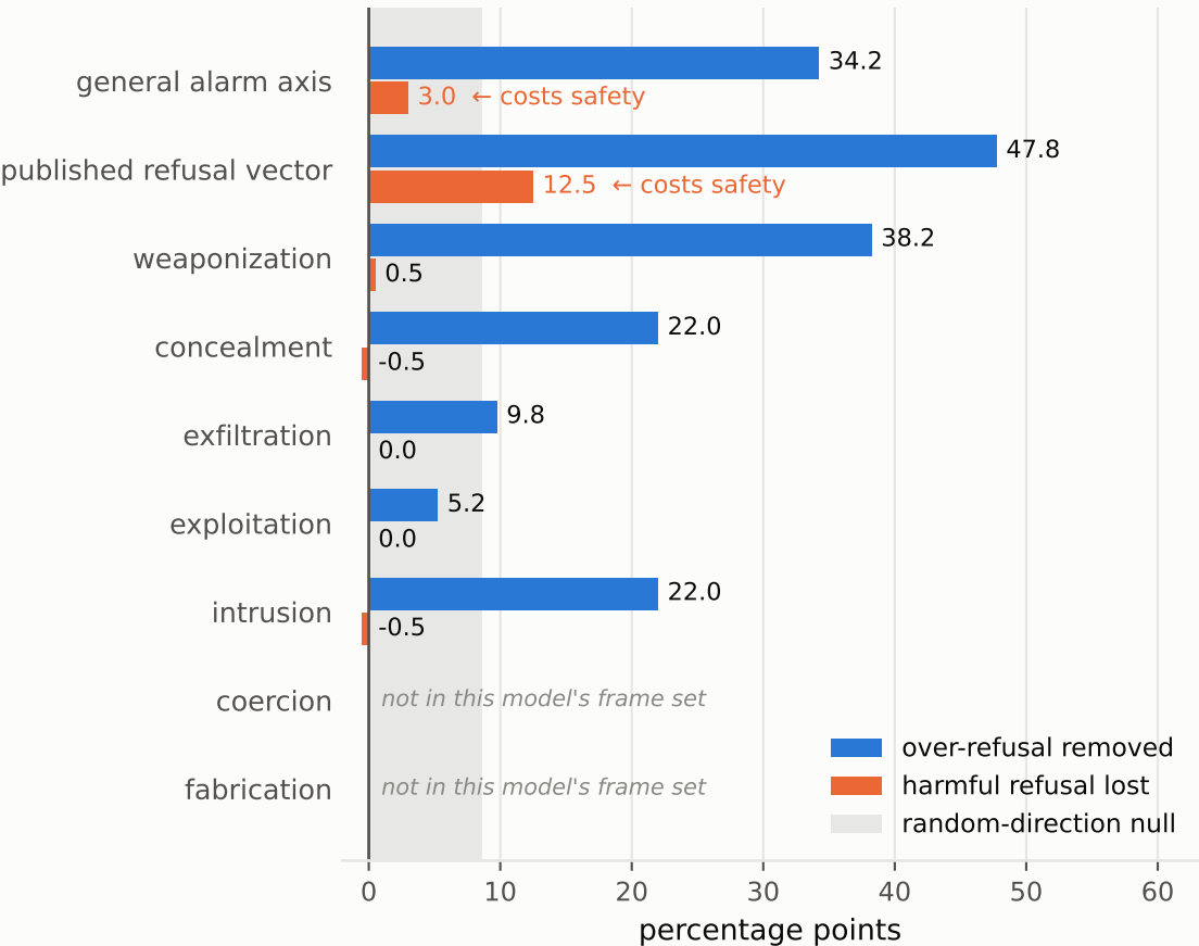
Llama-3-8B-Instruct
