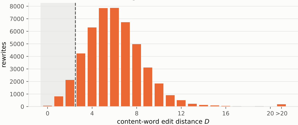
Qwen3-32B (n = 48,000 generated rewrites · D \leq 2 : 6.2%)
