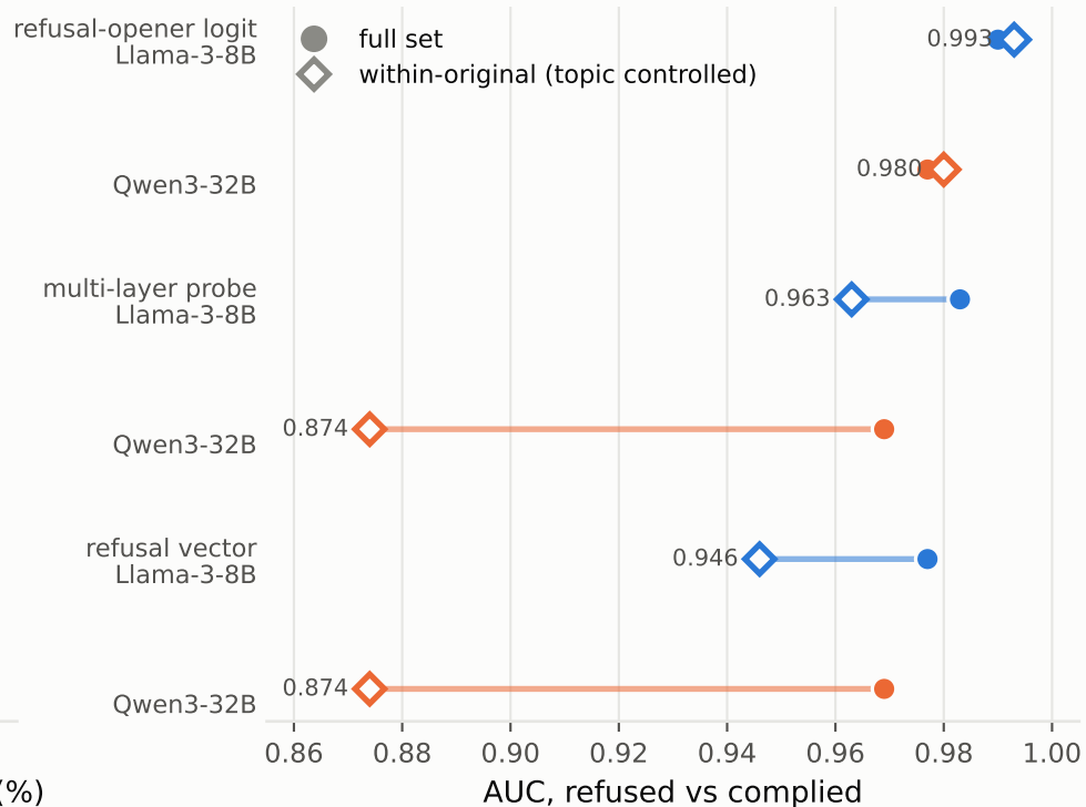
Controlling for topic separates the signals
