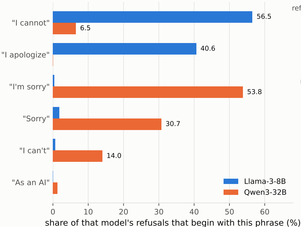
Refusal openers are model-specific
