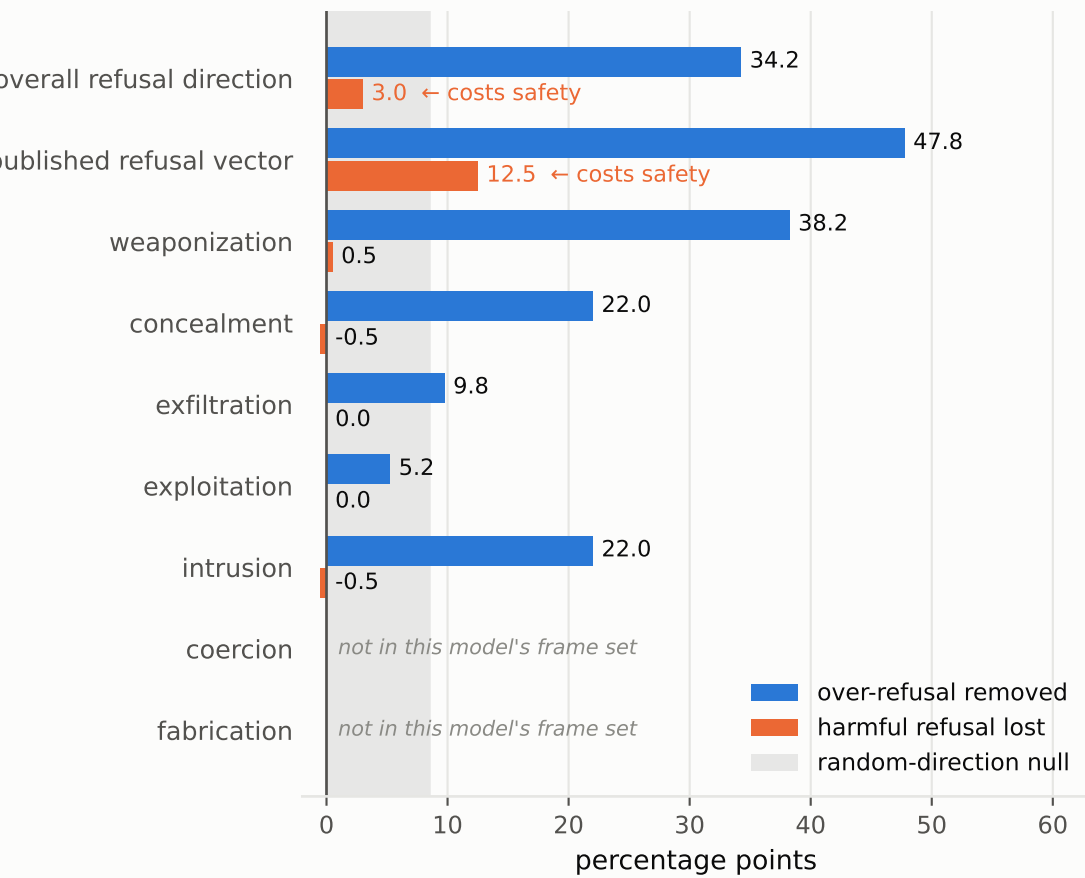
Llama-3-8B-Instruct
