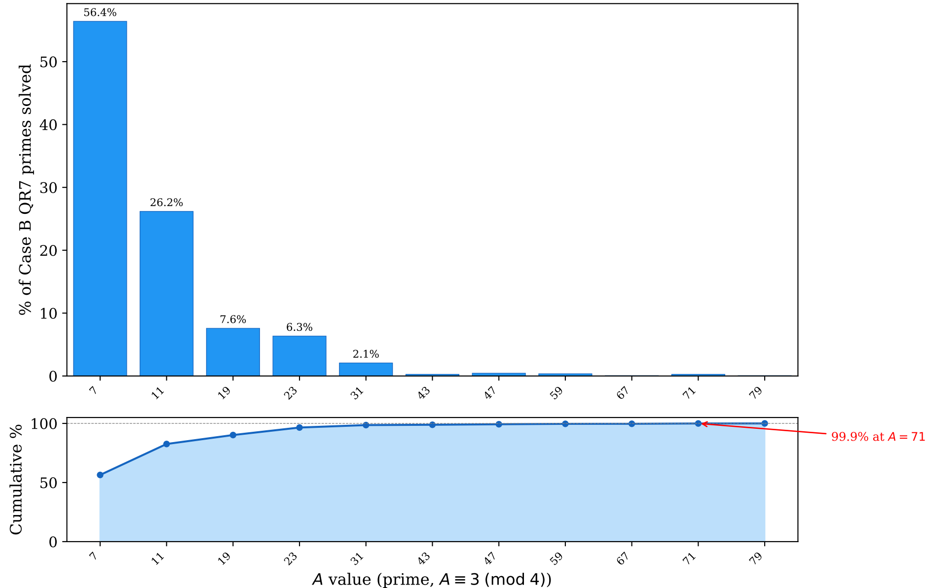
Distribution of first-working A value (2,269 Case B QR7 primes to 10^6 )
