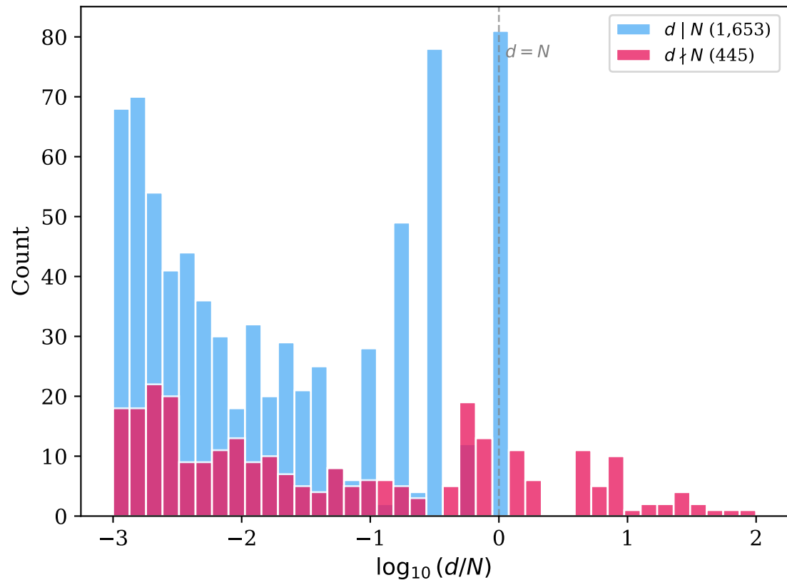
Distribution of d/N ratios
