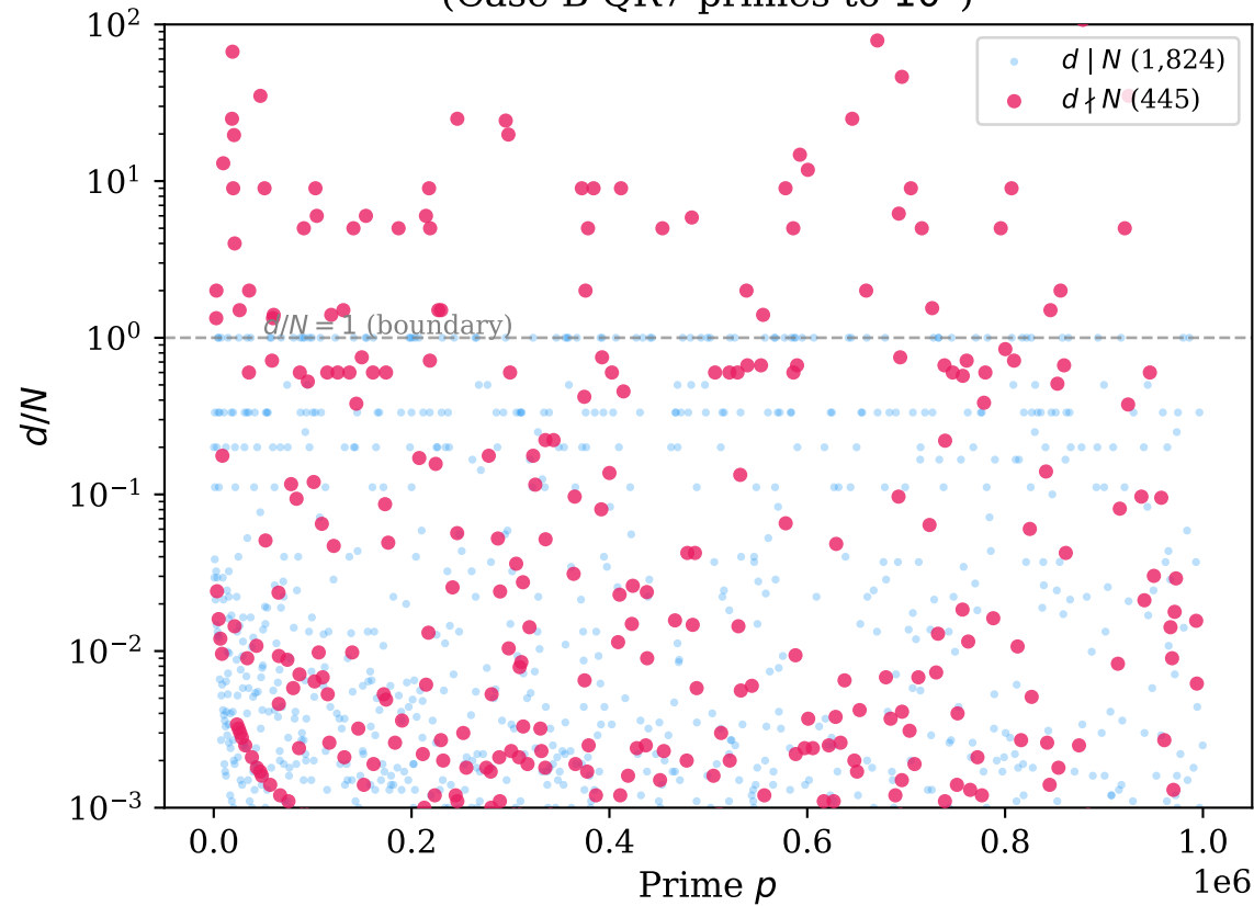
Gateway divisor ratio d/N (Case B QR7 primes to 10^6 )
