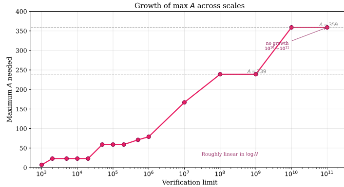
FIGURE 5. Maximum gateway parameter A required as the verification limit increases from 10^3 to 10^{11} . The growth is roughly logarithmic in the limit, in contrast with the factor-of- 10^8 increase in the search range.
