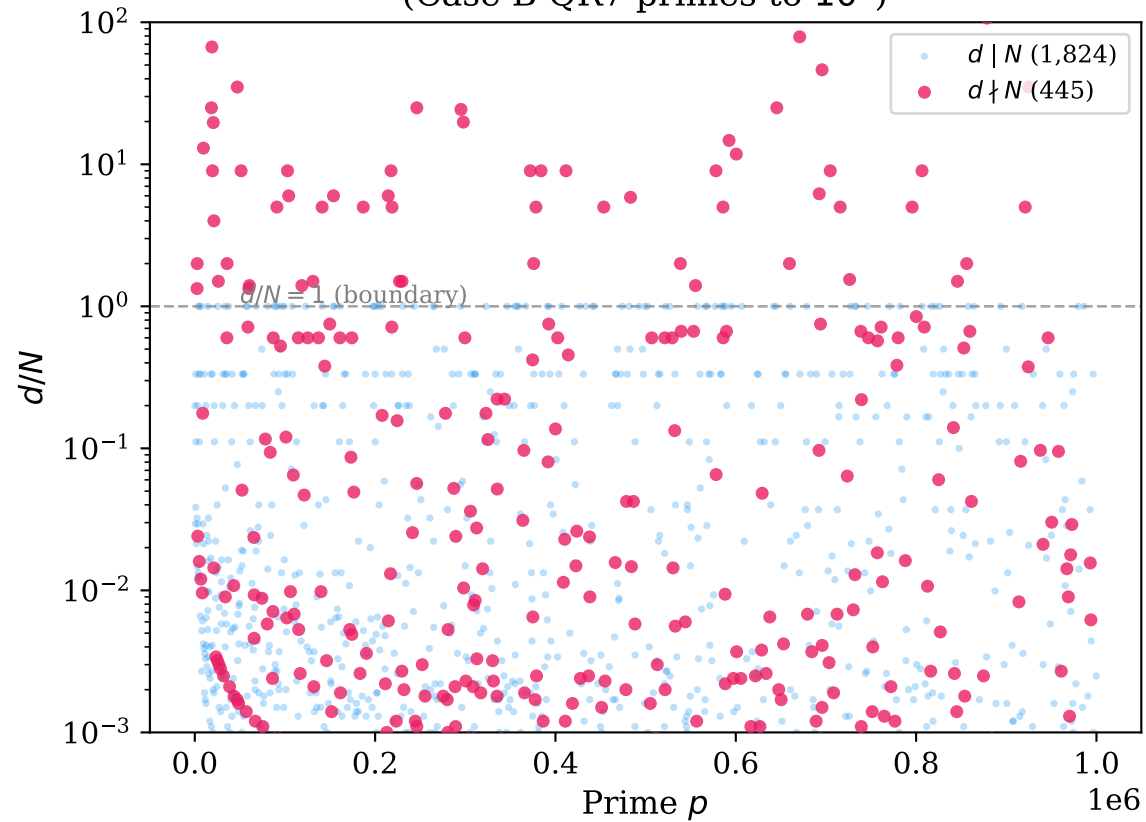
Gateway divisor ratio d/N (Case B QR7 primes to 10^6 )
