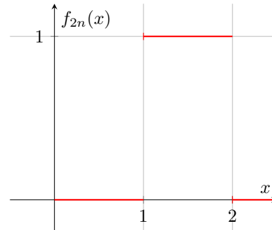
(b) f_{2n}(x) = \chi_{[1,2]}(x)
