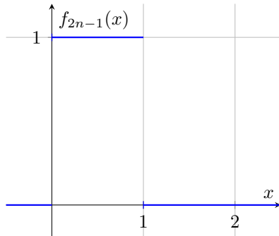
(a) f_{2n-1}(x) = \chi_{[0,1]}(x)
