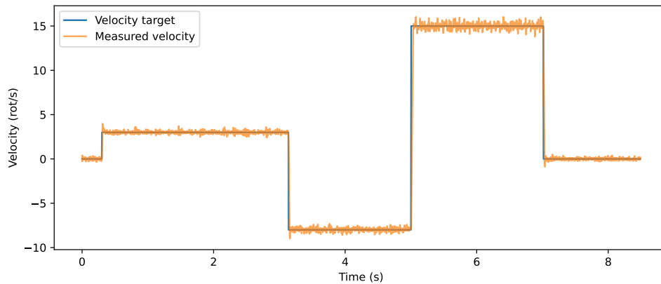
Figure 4.2: Velocity control
