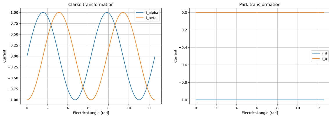
Figure 2.3: Park transformation of Clarke transformation output
