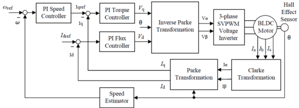
Figure 2.1: Field Oriented Control block diagram. [1]
