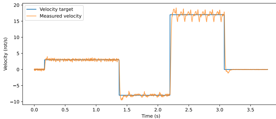
Figure 4.2: Velocity control
