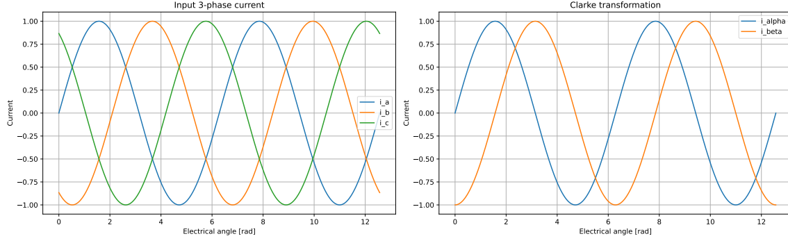
Figure 2.2: Clarke transformation of three-phase current.
