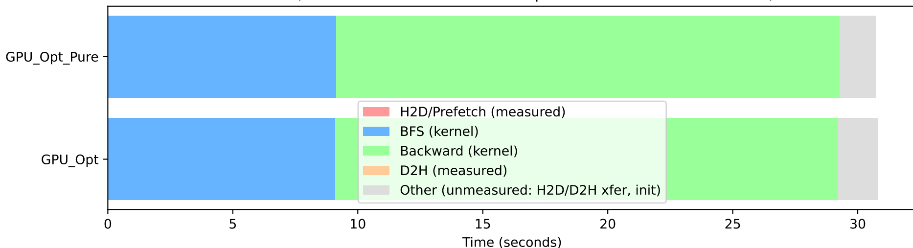
Phase Breakdown (BFS/Backward measured components + unmeasured Other): roadNet-CA
