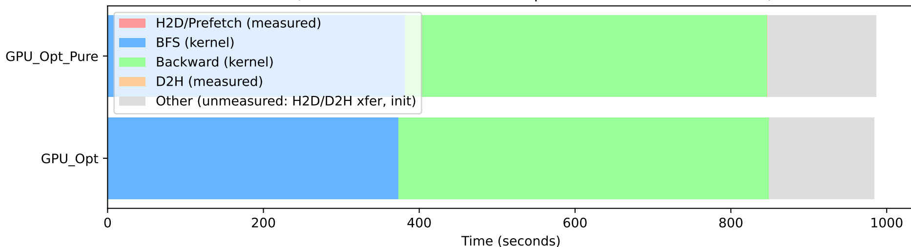
Phase Breakdown (BFS/Backward measured components + unmeasured Other): roadNet-TX
