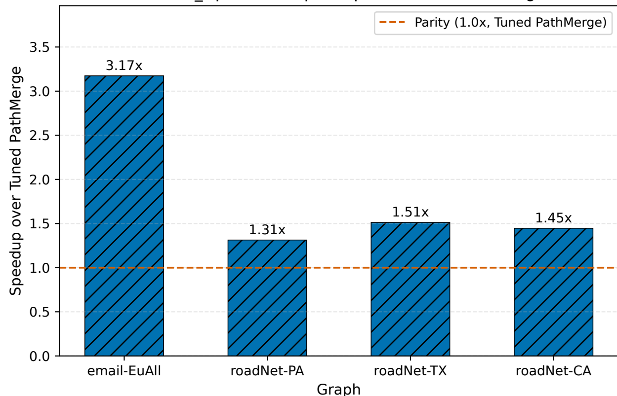
F2 GPU_Opt (b512) Speedup over Tuned PathMerge
