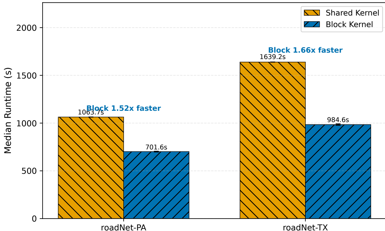
F6 Shared vs Block BFS Kernel (forced comparison)
