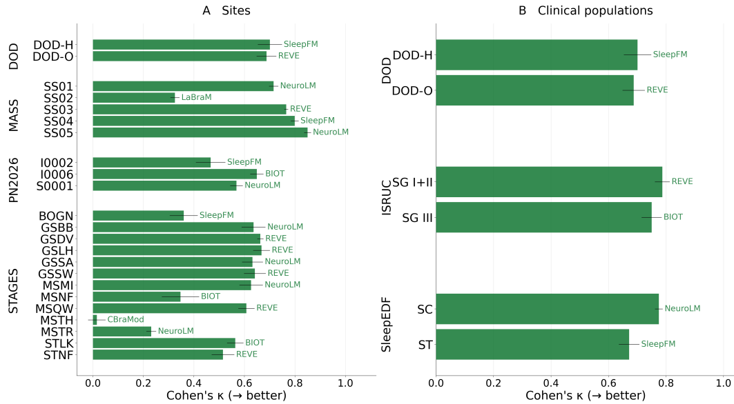
Figure 12: Cohen's \kappa sleep staging agreement for best performing EEG-FM per subset. (a) Subsets recorded at different sites differ significantly due to differing acquisition protocols. (b) Clinical cohorts are not systematically associated with lower performance. DOD-O contains patients with OSA, DOD-H contains healthy controls. ISRU Subgroup I and II contain patients with sleep disorders, Subgroup III contains healthy people. Parkinson's PD contains patients with Parkinson's disease, HOA contains healthy older adults. Sleep-EDF Cassette (SC) contains healthy patients, Telemetry (ST) contains medicated people.
