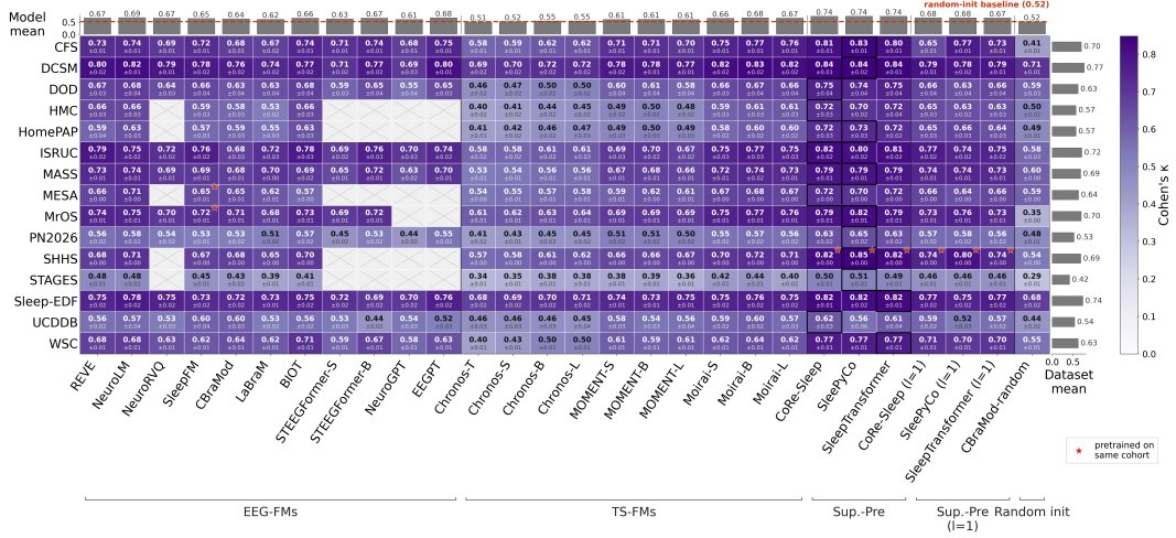
Figure 9: Sleep staging performance is strongly dataset-dependent. Cohen’s \kappa sleep staging agreement with ground-truth labels for all datasets and models per model category, i.e., EEG-FMs, TS-FMs, and Supervised-Pre models, with and without temporal context (sequence length l=1 ), and a random-initialized reference. Cohen’s \kappa (above) and standard deviation over folds (below) are shown for each. Black borders mark the cohort best-performing model. Red stars flag pretraining/evaluation overlap. Grey bars show mean performance over dataset and models respectively, with the red dashed line indicating mean random-initialized baseline. Missing results are indicated with a cross.
