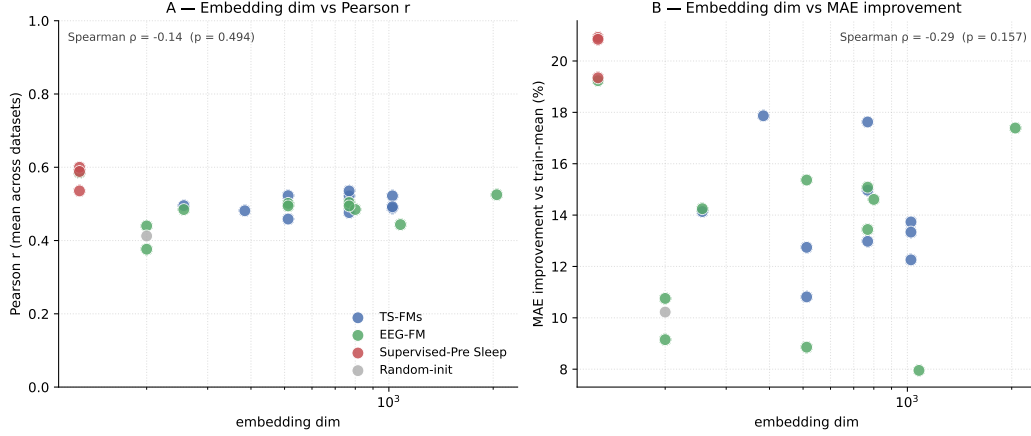
Figure 17: Embedding dimensionality does not correlate with brain-age performance. Each marker is one frozen-encoder checkpoint, with metrics fold-averaged across the seven main-pool brain-age cohorts (PN2026, WSC, ISRUC, SleepEDF SC, CFS, MrOS). Marker color denotes encoder family. (A) Embedding dim versus mean Pearson r between predicted and chronological age. (B) Embedding dim versus mean MAE improvement over a predict-cohort-mean baseline (%). The relationship is essentially flat in (A) (Spearman \rho = -0.14 , p = 0.49 ) and weakly negative in (B) ( \rho = -0.29 , p = 0.16 ).
