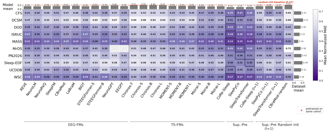
Figure 14: Sleep staging and hypnogram feature performance are not consistently aligned across datasets. Normalized Mean Absolute Error (MAE) between ground truth and predicted hypnogram features for all datasets and models per model category, i.e., EEG-FMs, TS-FMs, and Supervised-Pre models, with and without temporal context (sequence length l=1 ), and a random-initialized reference. Black borders mark the cohort best-performing model. Red stars flag pretraining/evaluation overlap. Grey bars show mean performance over dataset and models respectively, with the red dashed line indicating mean random-initialized baseline. Missing results are indicated with a cross.
