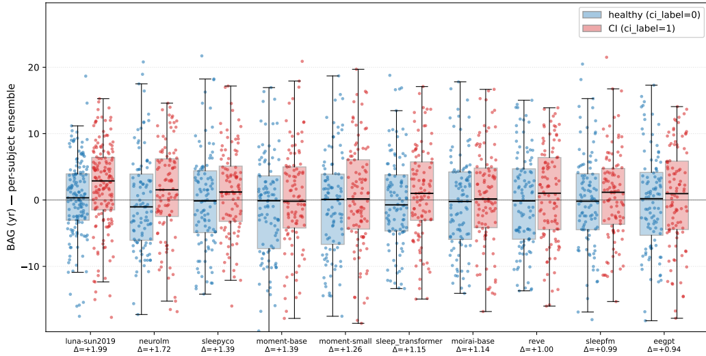
Figure 19: Brain-age-gap (BAG) distributions on the PN2026 Healthy/Cognitive Impairment holdout. BAG was computed per subject as predicted age minus chronological age using the 5-fold ensemble prediction. We show the 10 models with the largest positive mean BAG difference, ordered by \Delta \text{BAG} = \overline{\text{BAG}}_{\text{CI}} - \overline{\text{BAG}}_{\text{H}} . For each model, box plots show the BAG distributions of 100 age-matched healthy subjects and 100 cognitively impaired (CI) subjects; dots indicate individual subjects. The horizontal line marks \text{BAG} = 0 . Values below model names report \Delta \text{BAG} in years, where positive values indicate older-appearing EEG in the CI group.
