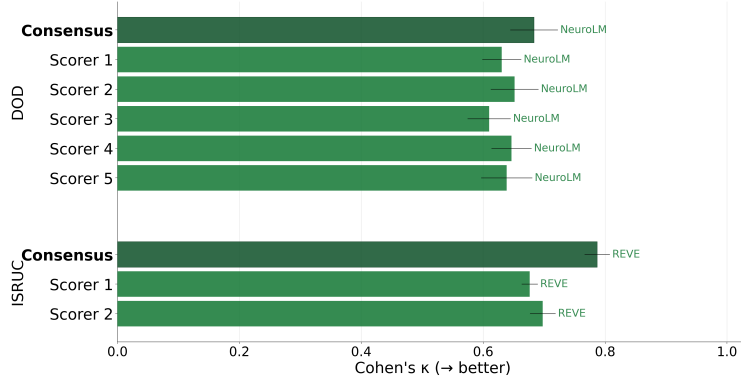
Figure 13: Sleep staging agreement is highest with consensus scoring, as ambiguous epochs are excluded. Cohen’s \kappa sleep staging agreement with ground-truth labels scored by different experts, and consensus scoring for best performing EEG-FM.
