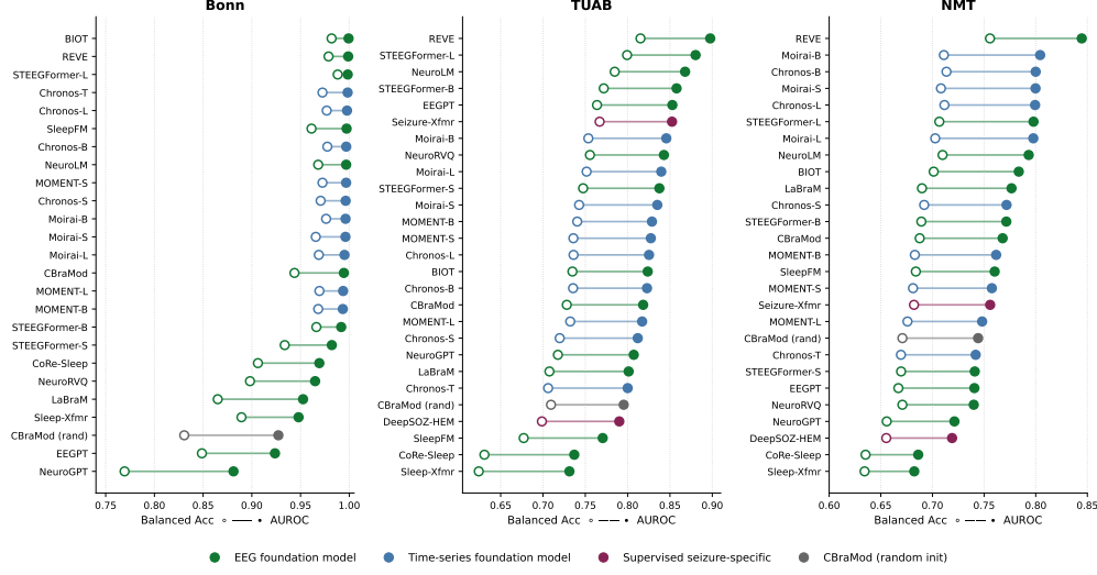
Figure 8: Foundation-model rankings on the three non-window EEG benchmarks (Bonn, TUAB, NMT). For each model and dataset, we plot AUROC (●) and balanced accuracy (○); the connector indicates the threshold-calibration gap (typically 0.05–0.11). Models are sorted within each panel by AUROC and colored by family: dark-green for general EEG foundation models, blue for time-series foundation models, burgundy for supervised seizure-specific baselines (SeizureTransformer, DeepSOZ-HEM), and grey for the CBraMod random-init ablation. All values are means over 5 stratified folds. REVE leads on all three datasets, Bonn is saturated, and NMT is the dataset on which TS-FMs come closest to parity with EEG-FMs.
