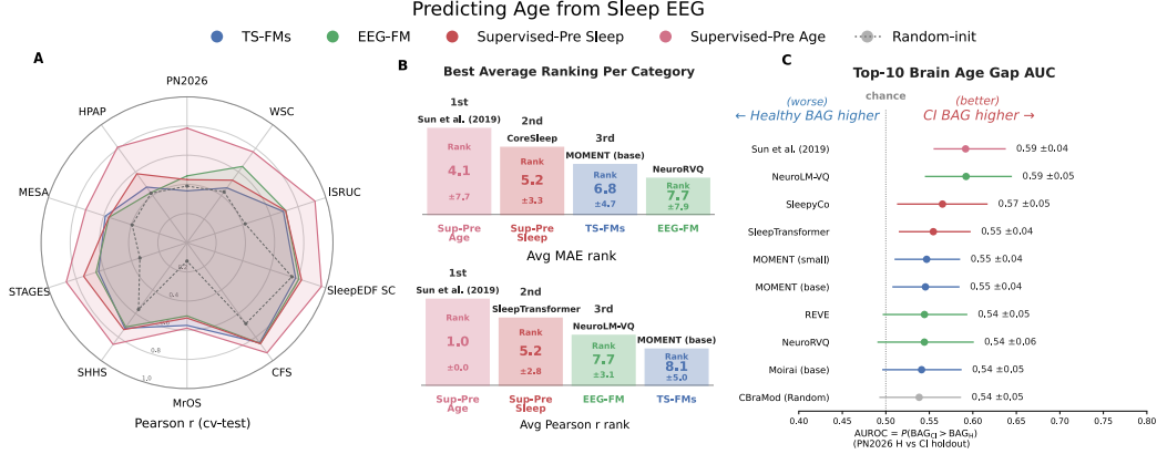
Figure 4: Supervised Models outperform EEG-FMs for Brain Age Prediction, but performance does not translate to neurodegenerative assessment biomarker. (A) Radar plot of performance (Pearson’s r ) of best model per category of models in different cohorts. Supervised Brain Age prediction outperforms the rest. (B) Best average ranking of the best model of each category for MAE and r metrics. (C) Top-10 AUROC for cognitive-impairment separation, using BAG (predicted minus chronological age). AUROC measures whether cognitively impaired subjects have higher BAG than age-matched healthy subjects. Although several models show weak positive separation, performance remains modest across model categories, indicating that accurate age prediction does not necessarily yield a robust BAG-based biomarker.
