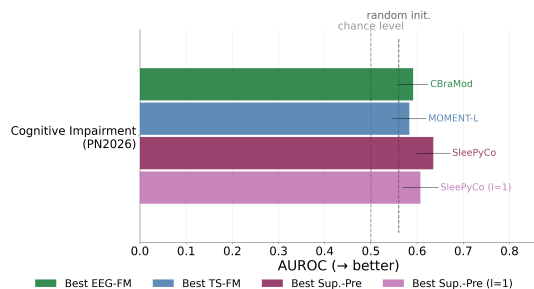
Figure 16: Models insufficiently encode cognitive impairment for reliable detection. Area under the receiver-operator curve (AUROC) for diagnosis of cognitive impairment in the PhysioNet 2026 dataset for best performing model per model category, i.e., EEG-FMs, TS-FMs, and Supervised-Pre models, with and without temporal context (sequence length l=1 ), and a random-initialized reference, is shown.
