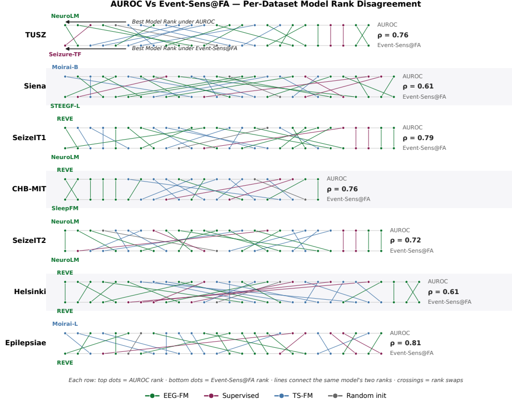
Figure 7: AUROC and event-level Sens@FA yield systematically different model rankings on every seizure-detection cohort. Each row corresponds to one cohort. Within a row, the upper rail of dots is the per-model rank by five-fold-mean window-level AUROC and the lower rail is the per-model rank by the event-based sensitivity-vs-FA/h AUC integrated over [0.1, 100] FA/h; rank 1 (best) is leftmost on both rails. Each line connects the same model’s two ranks, coloured by family (green: EEG foundation models; red: supervised pretraining; blue: time-series foundation models; grey: random initialisation). Every line crossing is a pair of models whose relative order flips between the two metrics. Spearman’s \rho between the two rankings (right of each row) ranges from 0.61 (Helsinki, Siena) to 0.81 (Epilepsiae) and is below 1 on every cohort, with mean \bar{\rho} \approx 0.72 across the seven cohorts. On TUSZ (top row, annotated), NeuroLM is rank-1 by AUROC but is overtaken by the supervised Seizure-TF model on Event-Sens@FA, illustrating that the conventional window-level metric selects a different model than the clinically relevant event-level one. 181 (cohort, model) pairs across the seven seizure-detection cohorts are shown.
