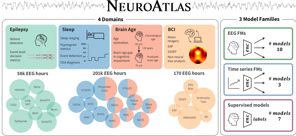
Figure 1: NeuroAtlas overview. NeuroAtlas spans four EEG domains (epilepsy, sleep, brain age, BCI) 42 datasets and \sim 260k hours of EEG, and benchmarks three model families on each. Per-domain task list and dataset coverage, with total EEG hours per domain (epilepsy: 58k h; sleep: 201k h, shared with brain age; BCI: 170 h). Each domain is evaluated with both standard and clinically grounded tasks: seizure detection with event-level decision metrics (epilepsy); sleep staging, hypnogram-derived features, event detection, and OSA diagnosis (sleep); chronological age estimation and the brain-age gap as a marker of cognitive impairment (brain age); and motor imagery, ERP, SSVEP, and non-neural confound analysis (BCI). Three model families compared under a unified frozen-encoder probe: 10 EEG foundation models, 3 time-series foundation model families, and 7 task-specific supervised baselines.
