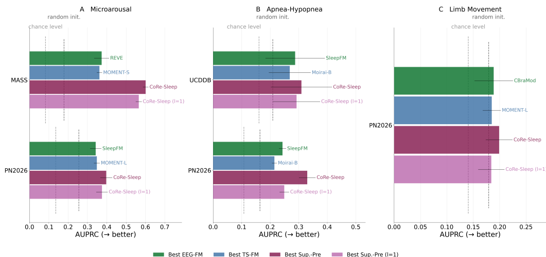
Figure 15: (FMs fail to adequately capture microarousals in their embeddings. Area under the precision-recall curve (AUPRC) for sleep event detection for best performing model per category. Prevalence indicates chance baseline. (a) Microarousals with a minimal duration of 3 seconds. (b) Apnea and hypopnea events with a minimal duration of 10 seconds. (c) Periodic limb movement with a minimal duration of 0.5 seconds.
