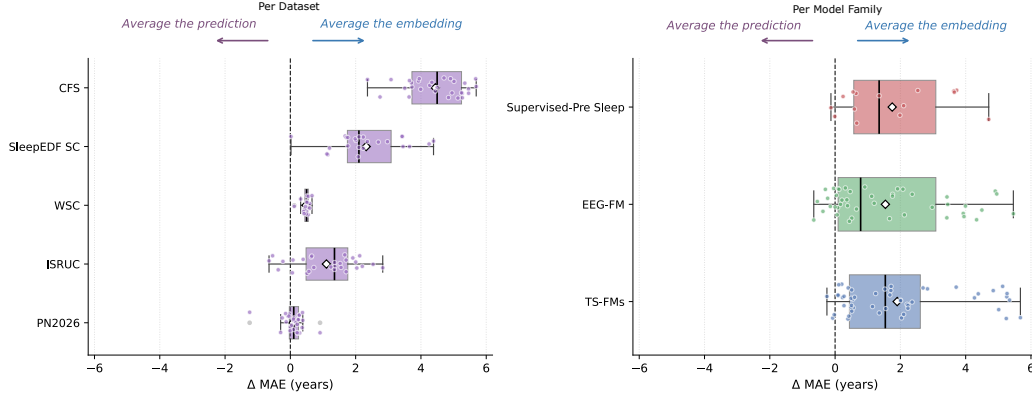
Figure 18: Aggregating per subject tends to outperform aggregating per epoch. Each marker is one (model, cohort) pair, fold-averaged across the 5 folds; The horizontal axis shows \Delta \text{MAE} = \text{MAE}_{\text{epoch}} - \text{MAE}_{\text{subject}} ; positive values indicate that subject-level Ridge (mean-pool a recording’s epoch embeddings into one subject vector before fitting to age beats epoch-level Ridge fit per 30s epoch, then average predictions per subject). (left) Per-cohort distributions, ordered by n_{\text{outer\_train}} ascending;
