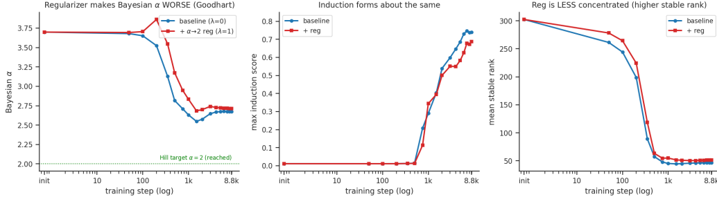
Figure 7: Causal test of the \alpha \rightarrow 2 regularizer (seed-matched pair; only the regularizer differs). Left: the regularizer reaches its Hill target ( \alpha = 2 , green) but makes the Bayesian \alpha worse (red above blue throughout)—a Goodhart hack the posterior detects. Center: induction forms about the same in both arms. Right: the regularized spectrum is less concentrated (higher stable rank). \alpha is a readout of training, not a lever: forcing it neither matures the spectrum (by the rigorous measure) nor builds the circuit.
