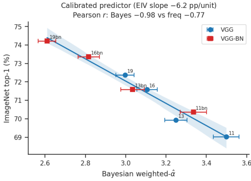
Figure 2: VGG weighted- \hat{\alpha} as a calibrated accuracy predictor. The errors-in-variables regression propagates per-model \hat{\alpha} posterior uncertainty (horizontal error bars); the band is the 95% predictive interval. The posterior \hat{\alpha} tracks accuracy ( r = -0.98 ) more strongly than the frequentist ( r = -0.77 ).
