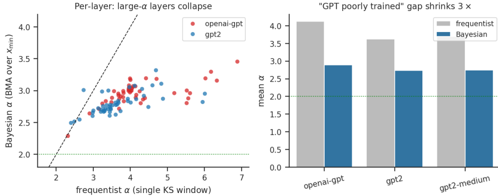
Figure 1: The GPT/GPT2 “training quality” gap is largely a scaling-window artifact. Left: each point is one weight matrix; the frequentist \alpha (single KS window) versus the wwjd posterior \alpha (Bayesian model-averaged over x_{\min} ). Layers the point estimate calls “unusually large” ( \alpha > 5 ) collapse toward \alpha \approx 3 . Right: mean \alpha per model; the frequentist gap that underwrites “GPT is poorly trained” shrinks 3.1\times under the posterior.
