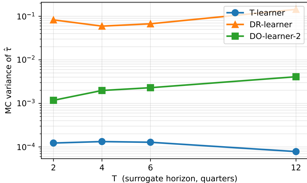
Estimator MC variance vs T
