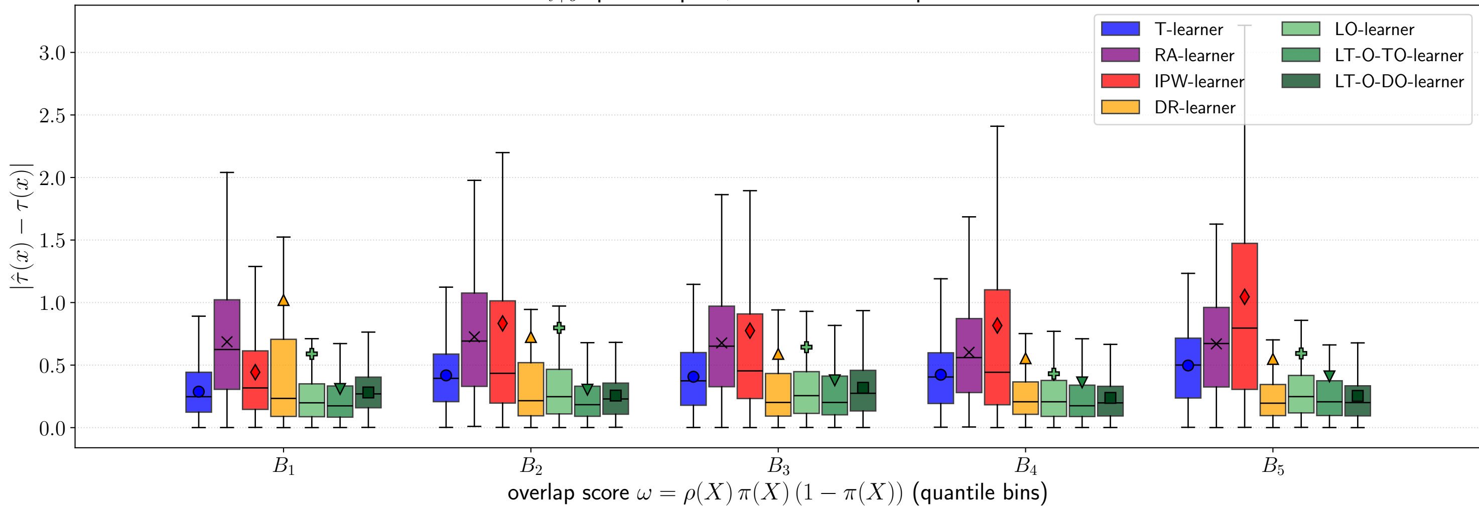
\mathcal{D}_{t+o} : per-sample \sqrt{\text{PEHE}} vs. overlap-score bin
