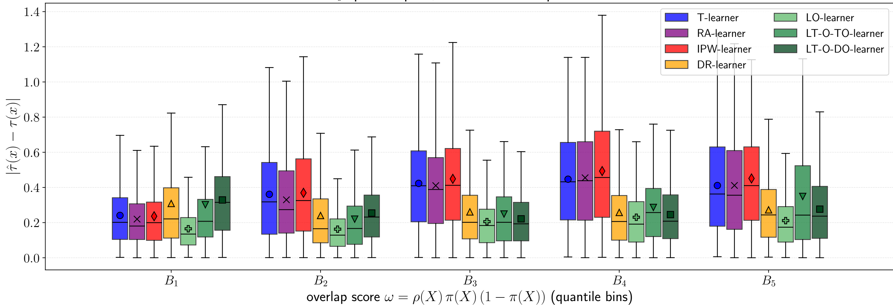
\mathcal{D}_o : per-sample \sqrt{\text{PEHE}} vs. overlap-score bin
