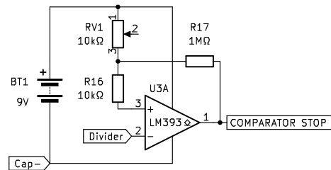
Comparator Circuit
