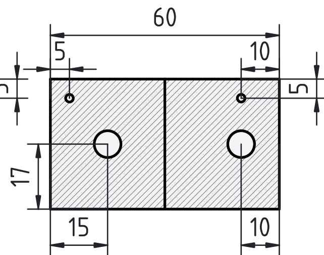
Busbar #3
