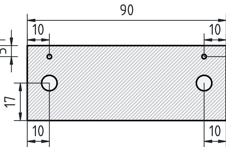
Busbar #2
