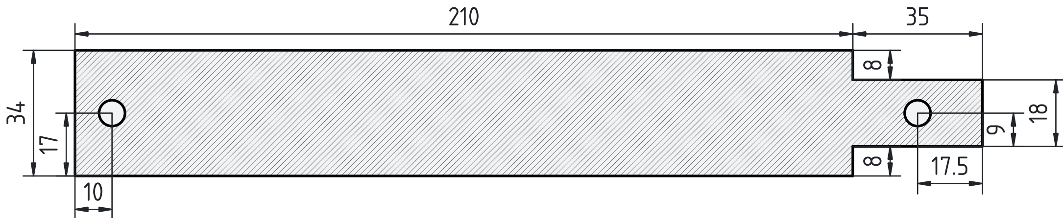
Busbar #4
