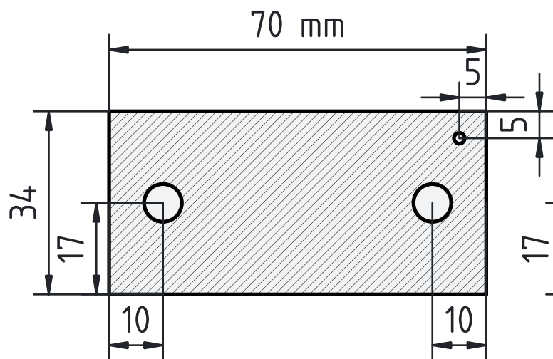
Busbar #4
