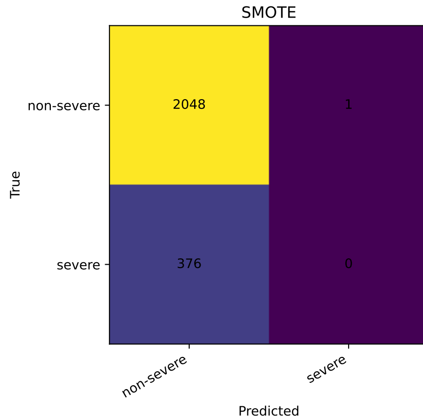
Confusion Matrix Comparison (Counts)
