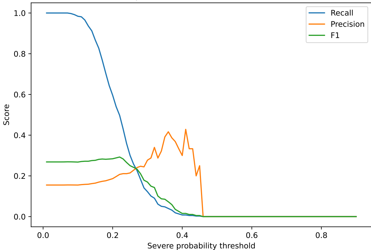
Threshold Optimization (SMOTE) — Severe accidents
