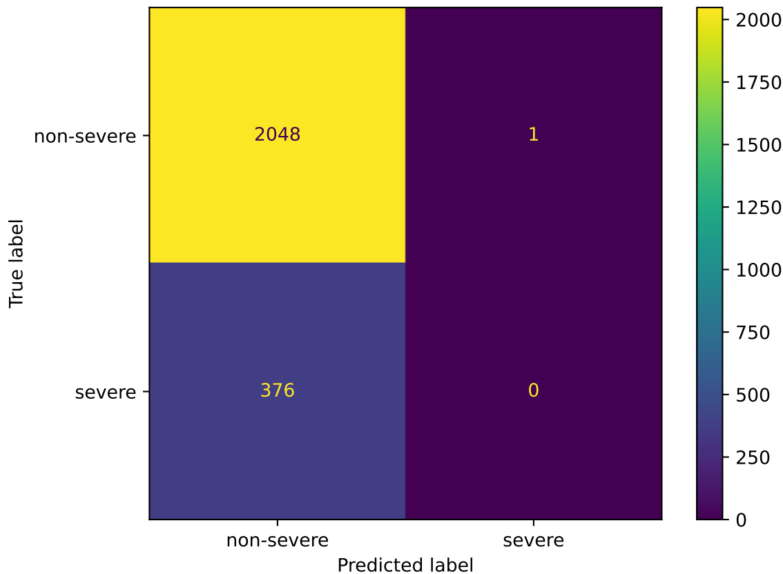
Confusion Matrix — SMOTE (default threshold)
