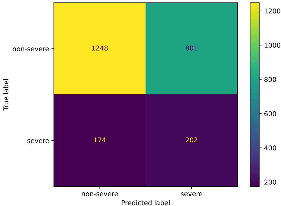
Confusion Matrix — SMOTE + Threshold override
