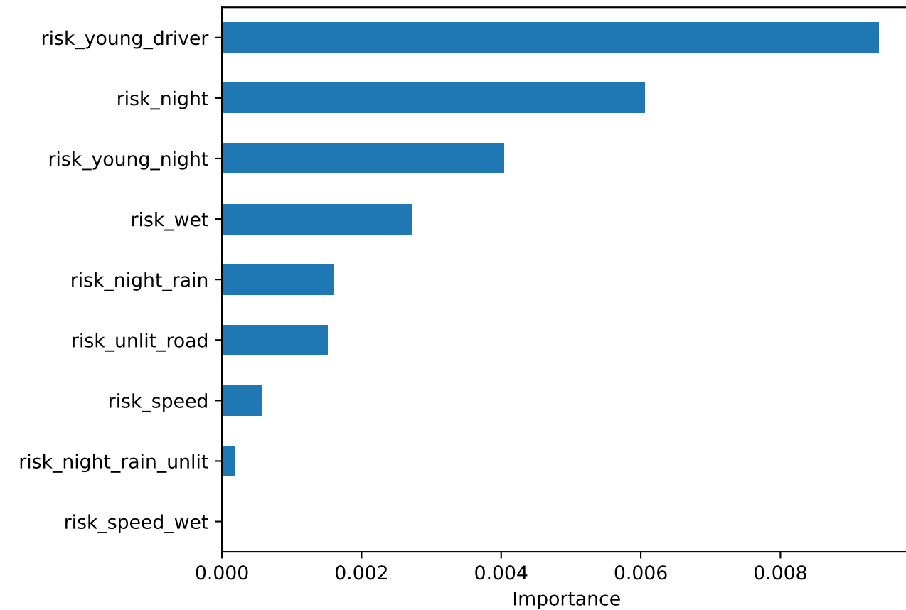
Risk Features — SMOTE
