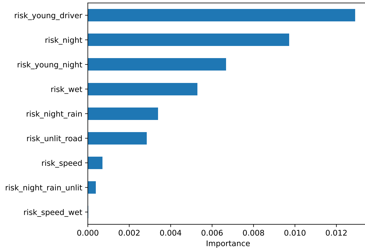
Risk Features — Baseline
