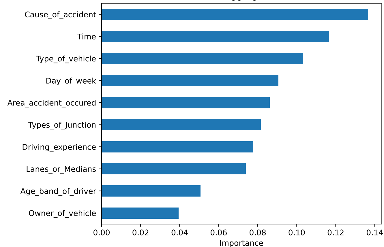
Risk Features — SMOTE
