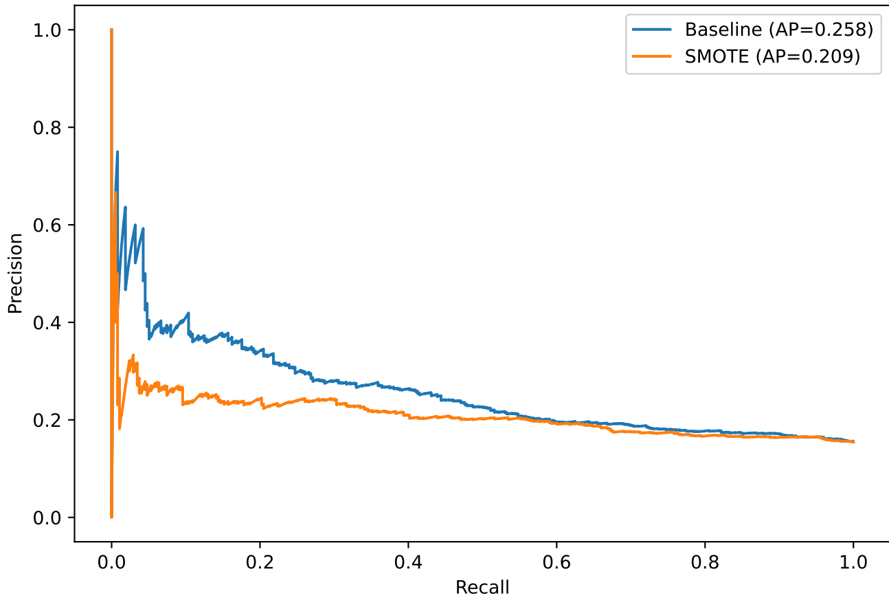
Precision-Recall Curve (Severe = fatal+serious)
