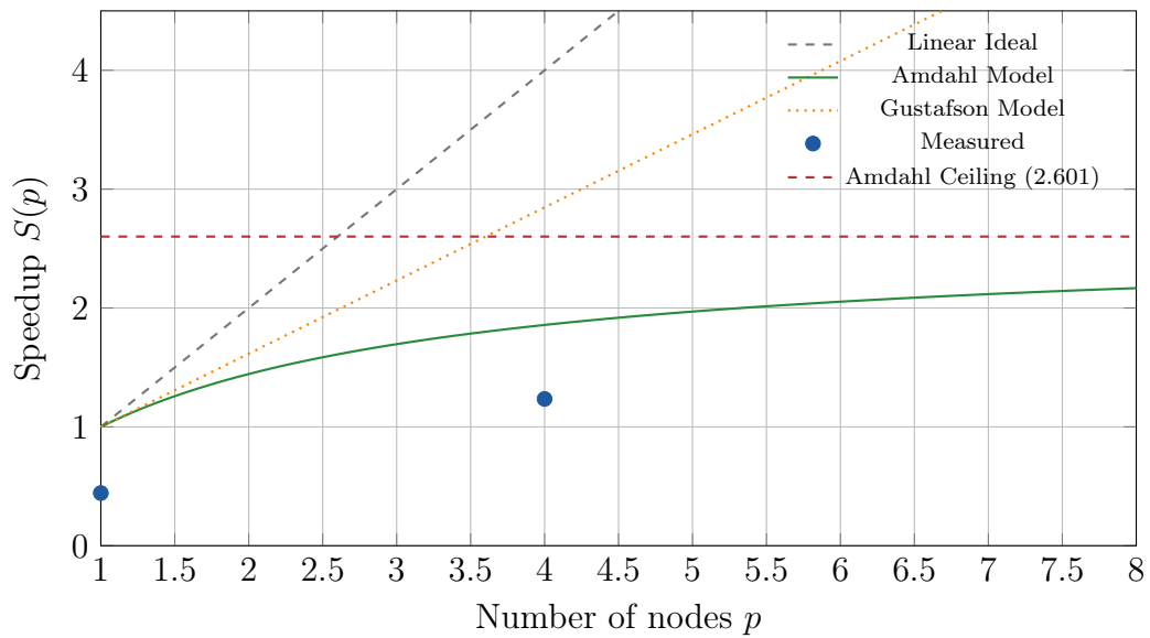
Figure 1: Speedup comparison between theoretical models and measured MPI performance on the Raspberry Pi cluster. The measured points lie well below Amdahl's prediction, confirming severe network-bandwidth limitation.
