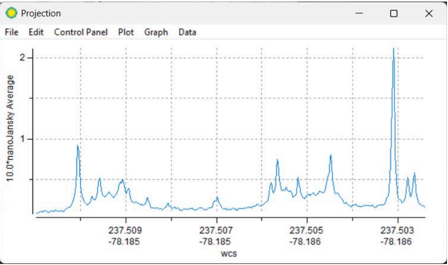
2D linear section of an area of the dataset, plotting emission peaks.
