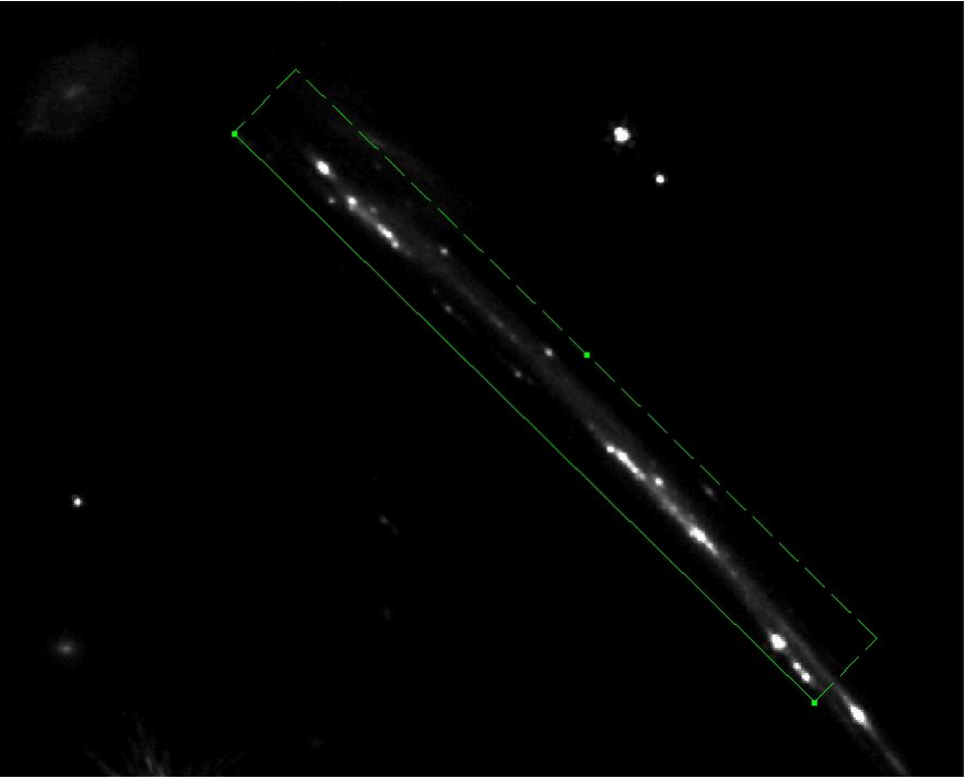
A newborn galaxy, roughly 11 billion years ago, warped and observable thanks to a gravitational lens curving light.
