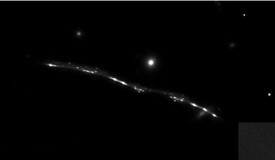
A newborn galaxy, roughly 11 billion years ago, warped and observable thanks to a gravitational lens curving light.
